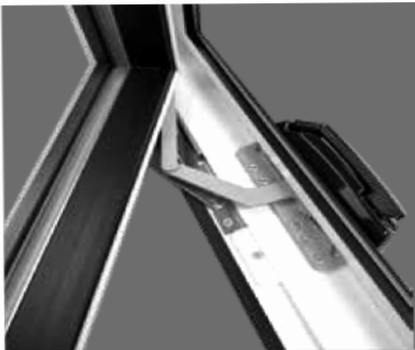
Heavy Duty Casement Crank Mechanism
